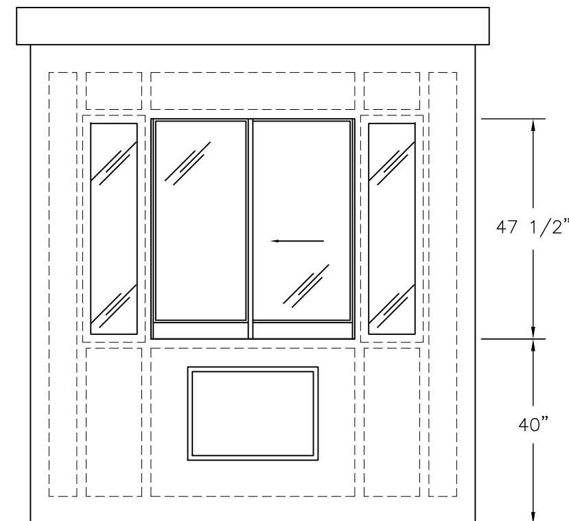
ELEVATION D
