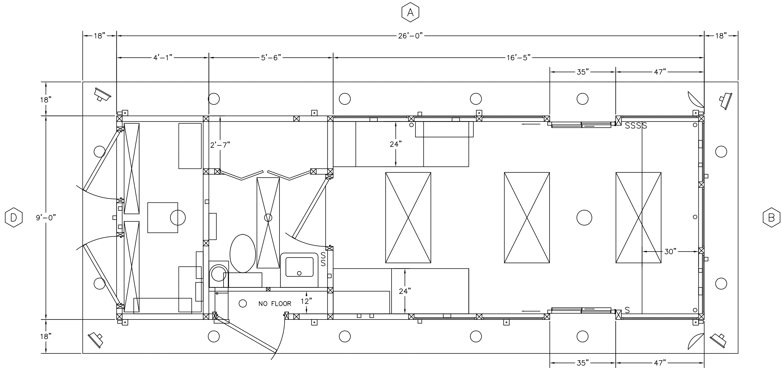
C PLAN VIEW RESTRICTED AREA GUARD HOUSE
