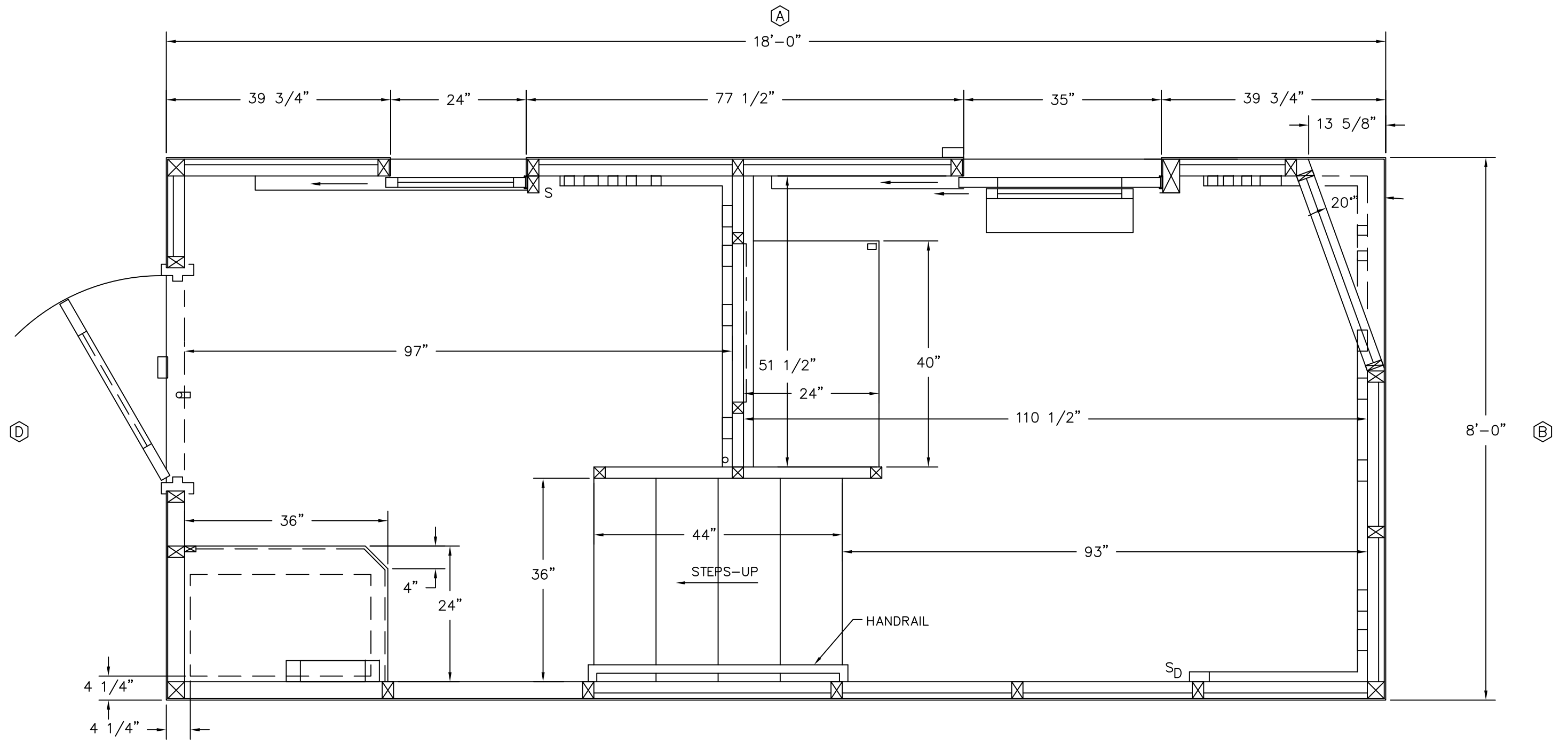
PLAN VIEW
