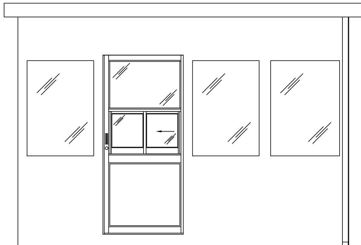
ELEVATION C
