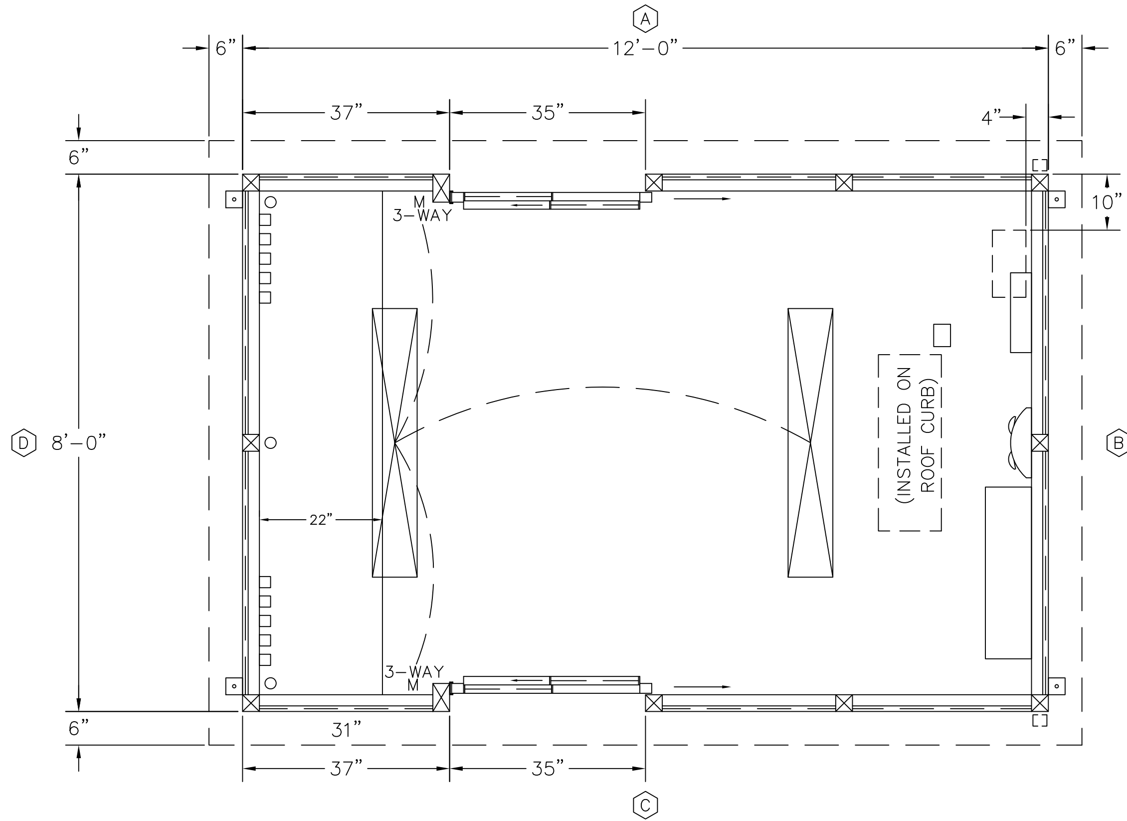
PLAN VIEW
