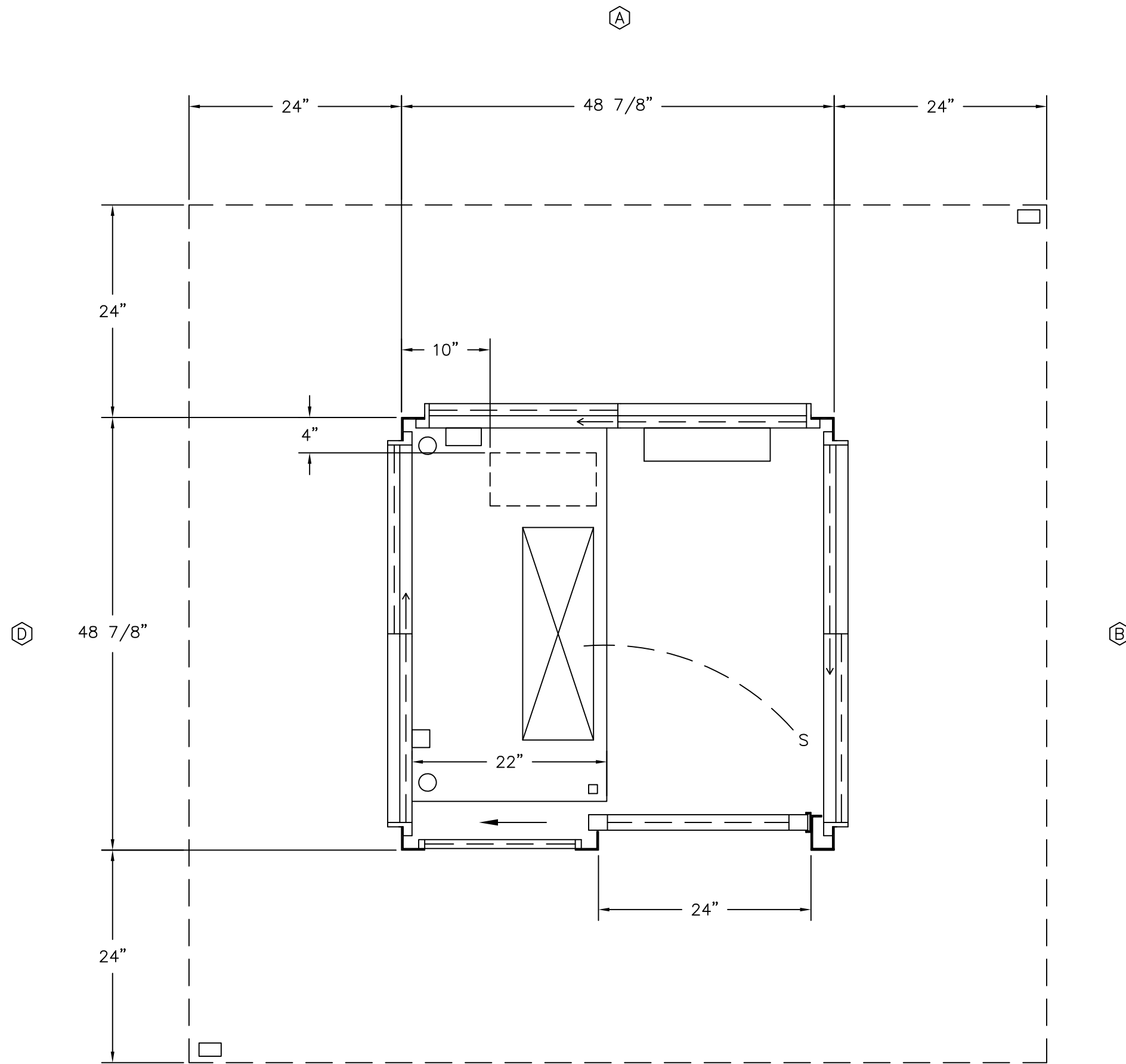
PLAN VIEW
