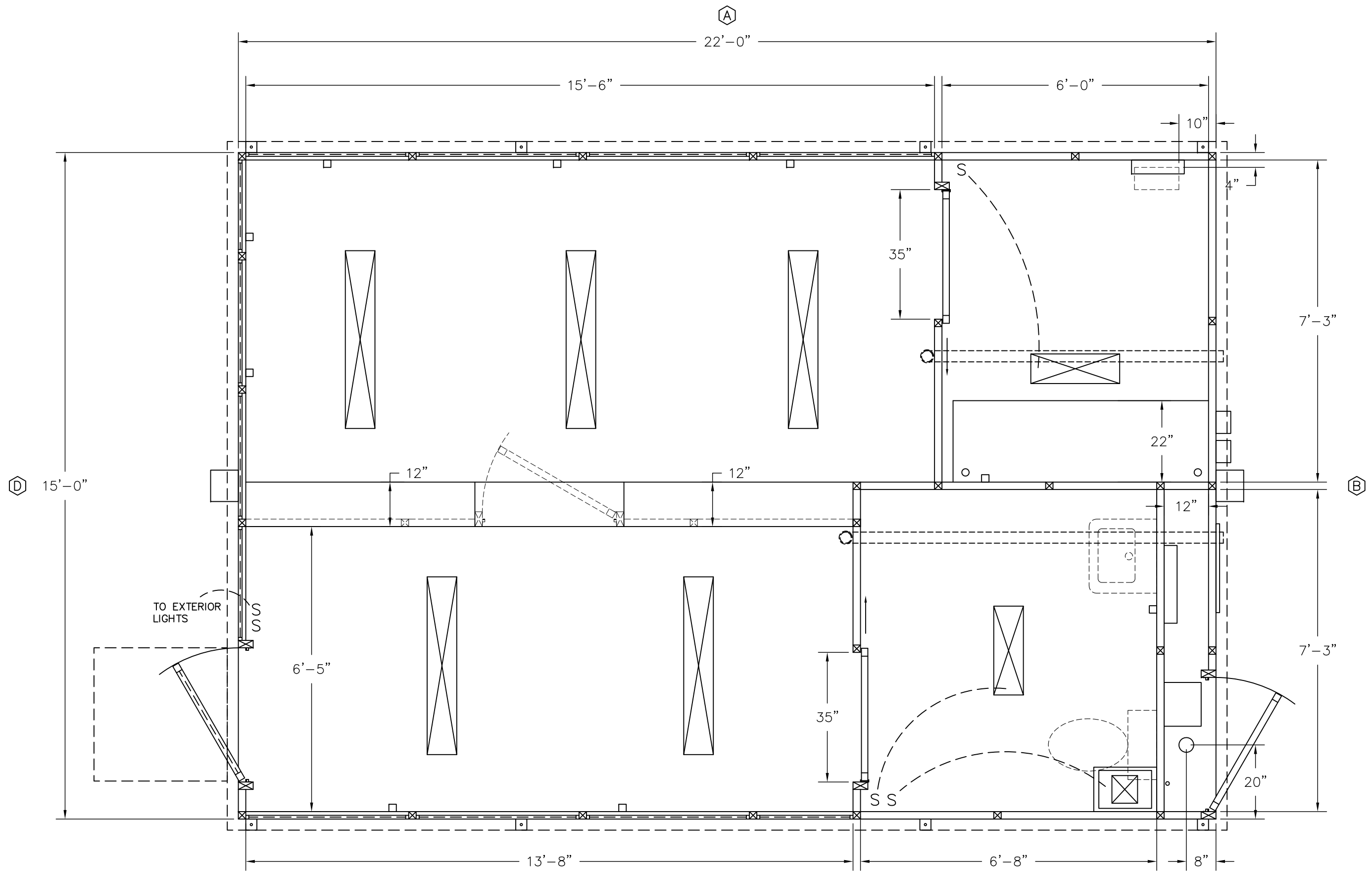
PLAN VIEW
