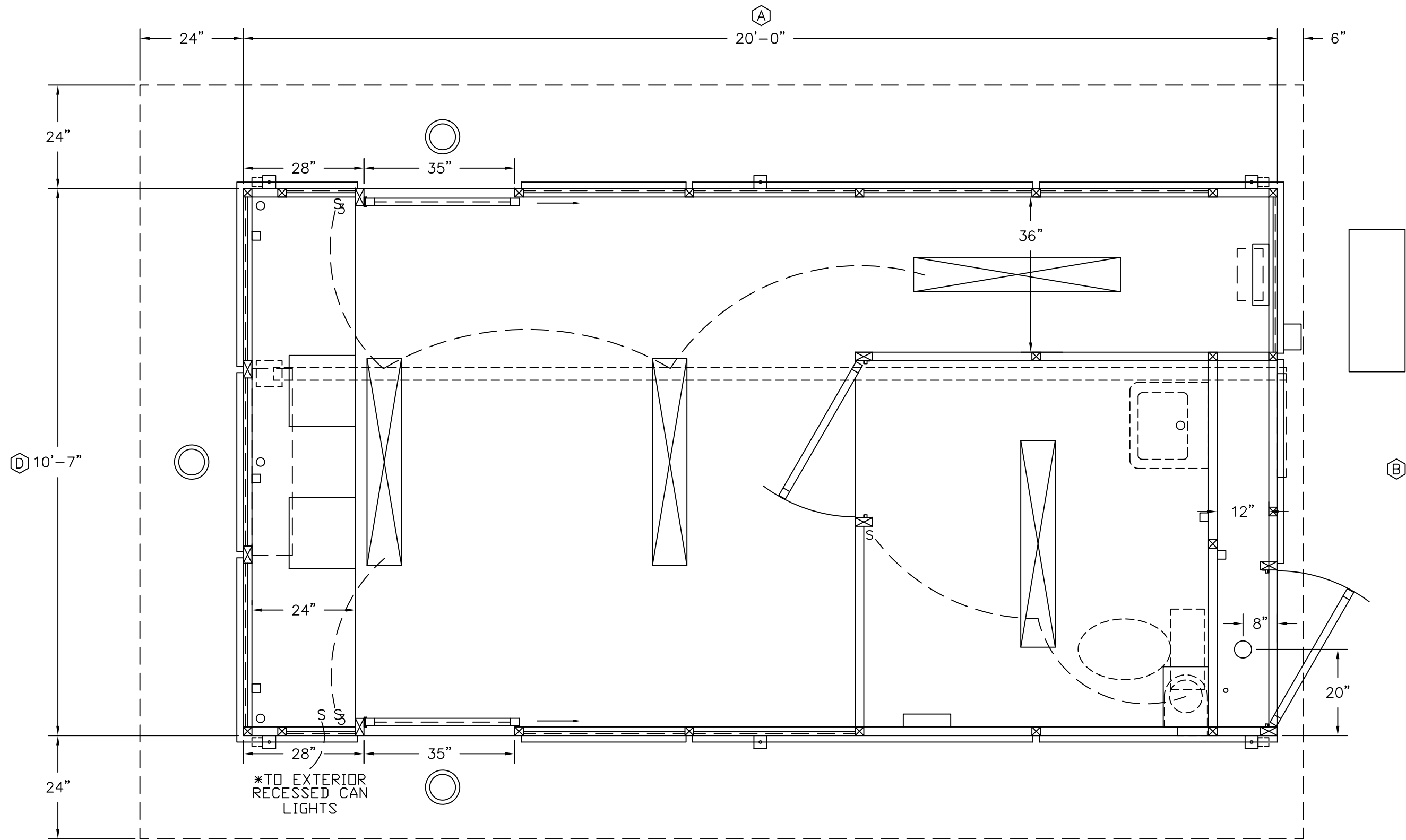
(C) PLAN VIEW
