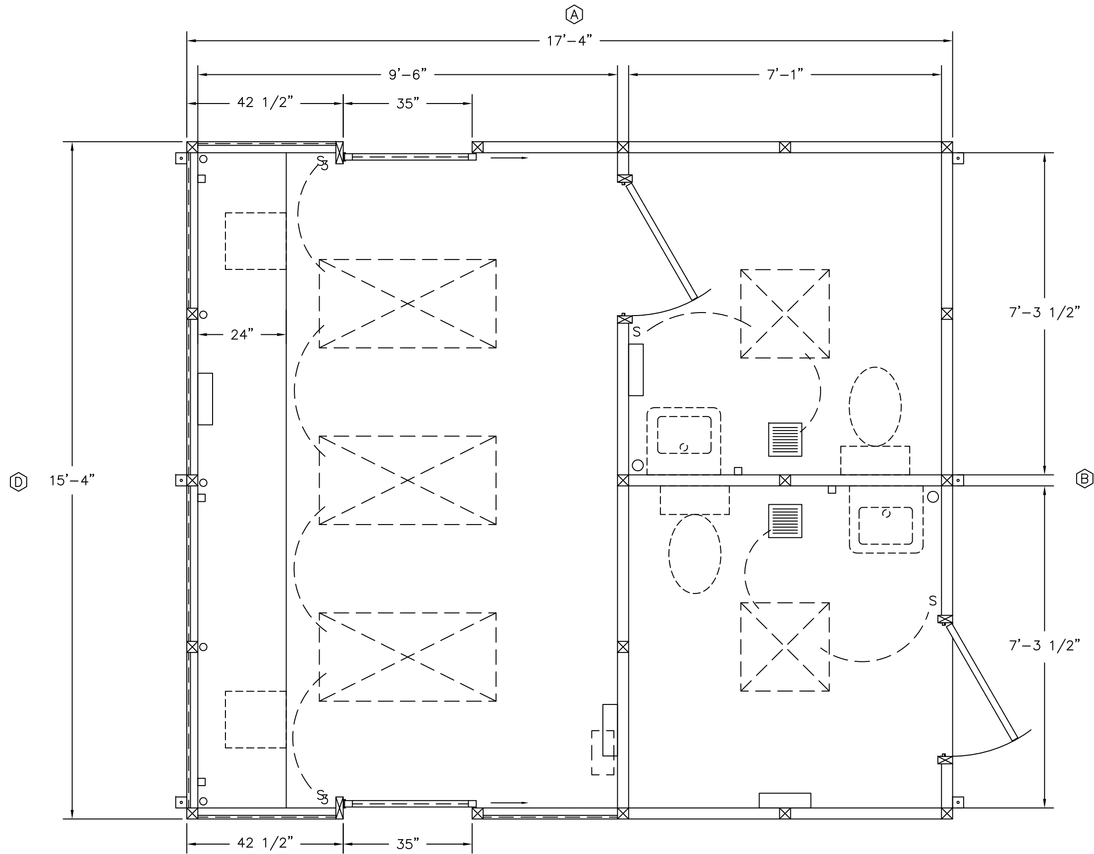
(C) PLAN VIEW
