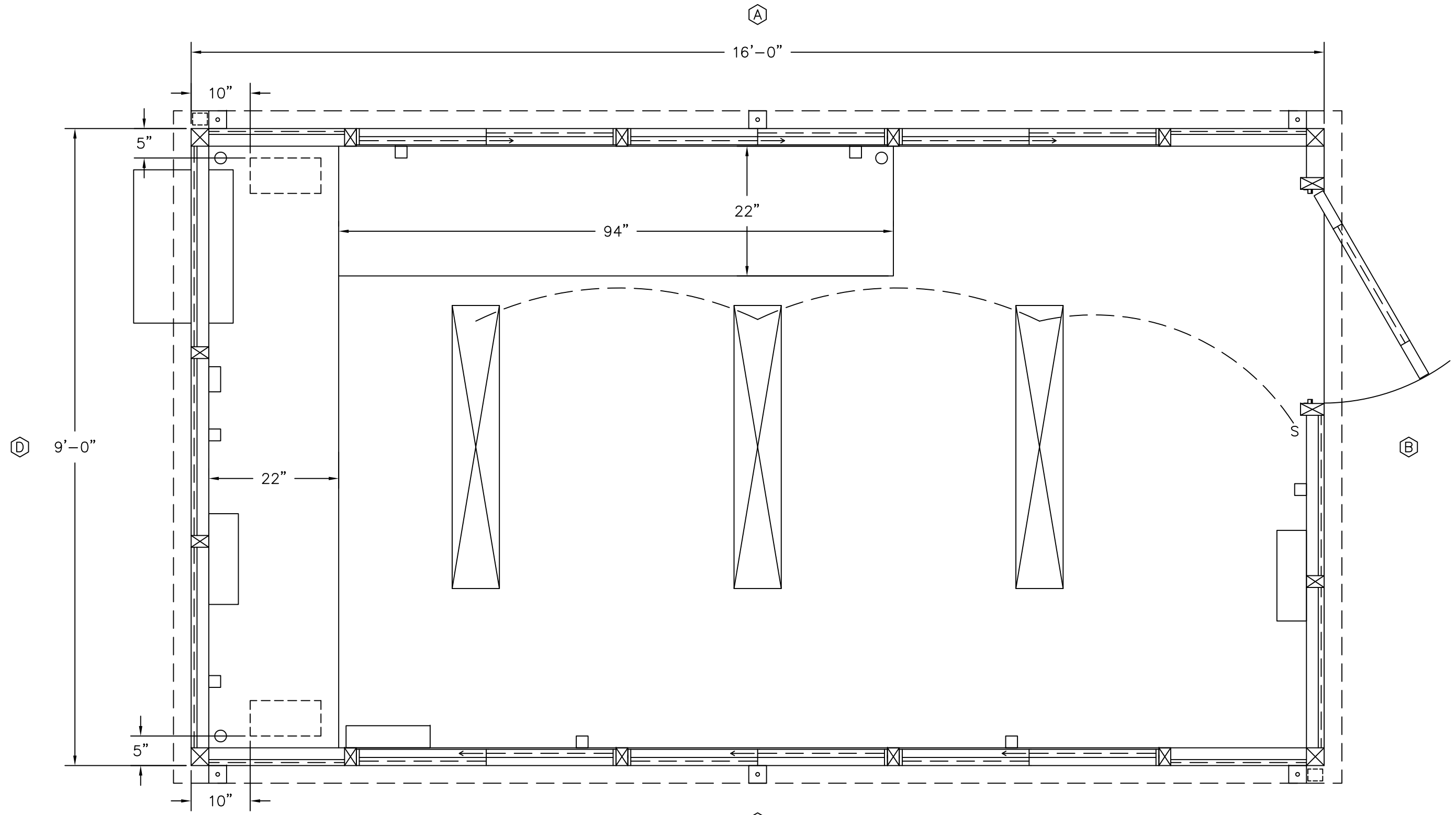
PLAN VIEW
