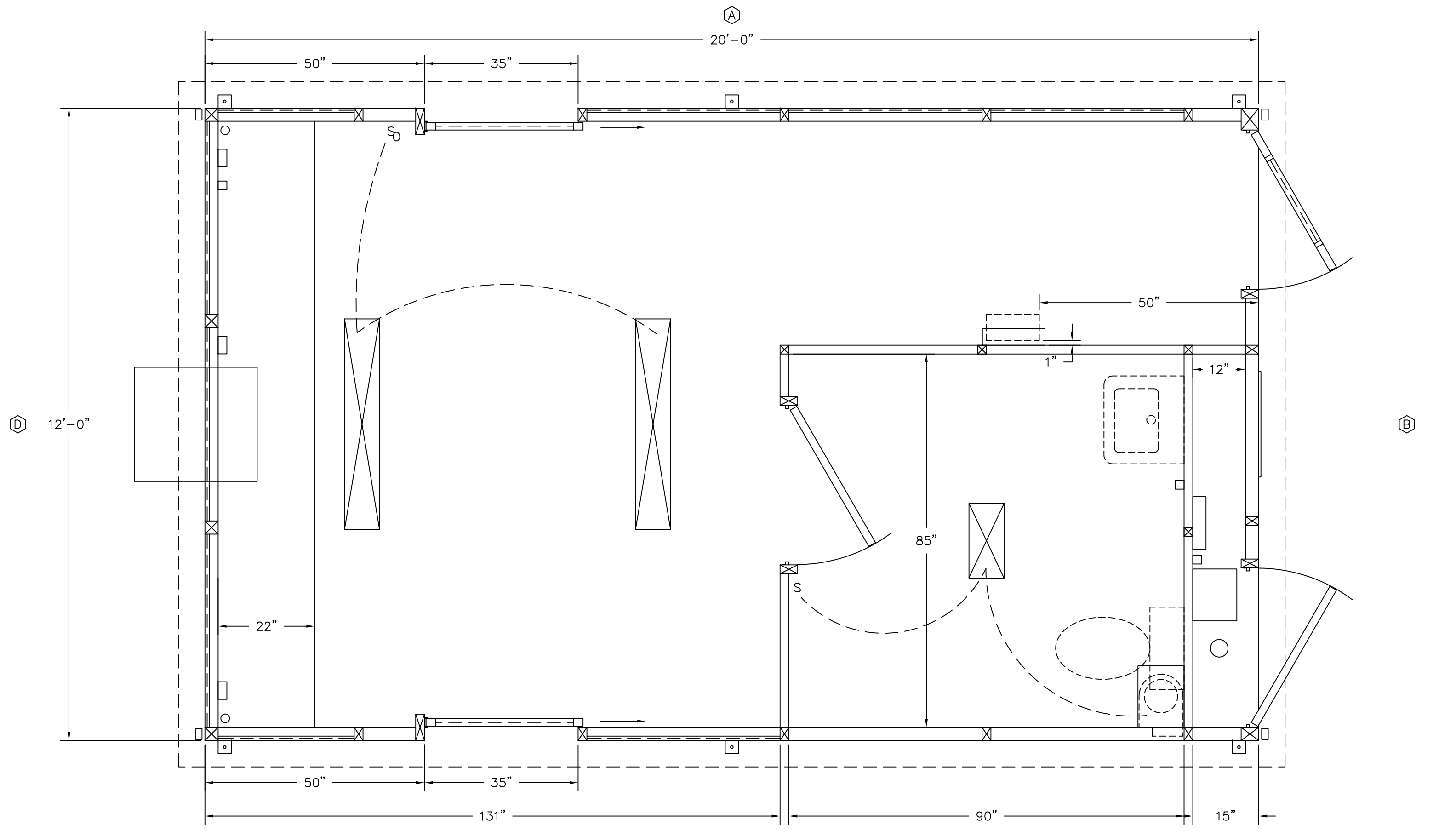
PLAN VIEW
