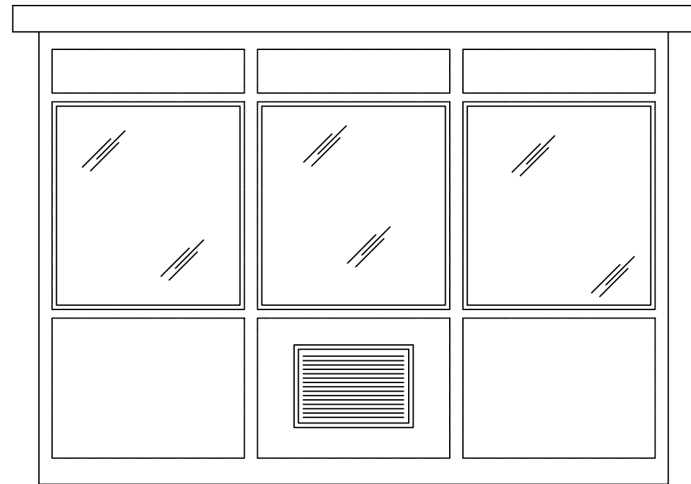
ELEVATION D
